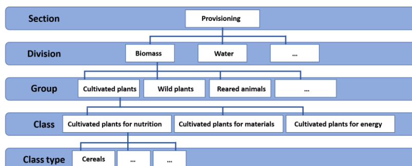
Figure 1. Diagram of the CICES taxonomy
